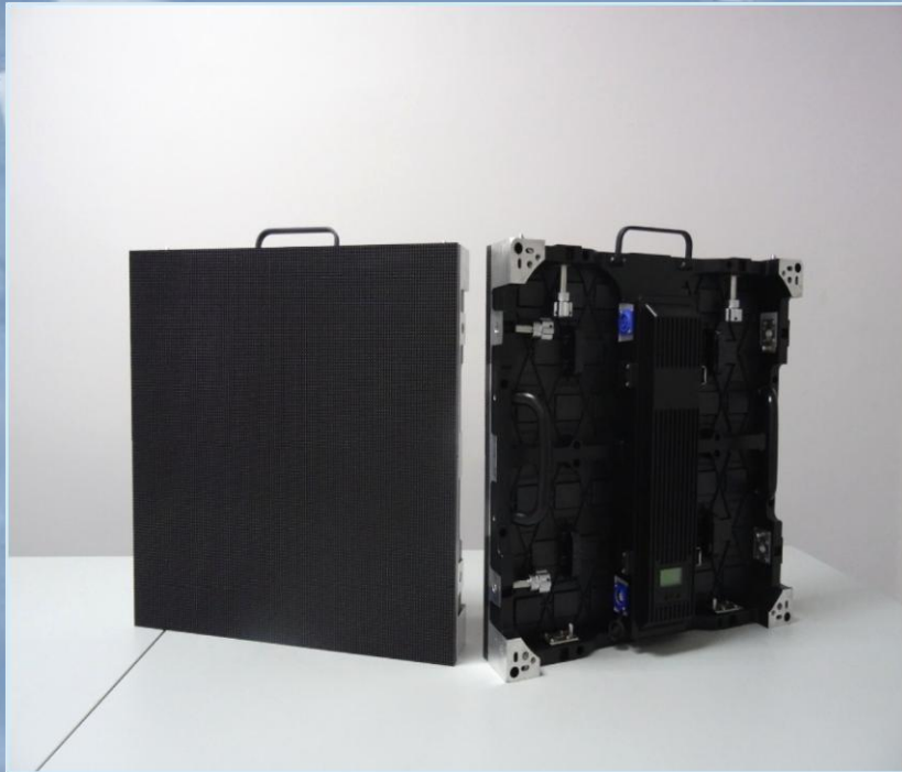
Die-casting aluminum cabinet
